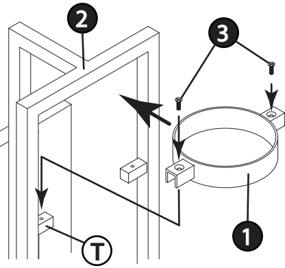
DRAWING 2 - ASSEMBLY
