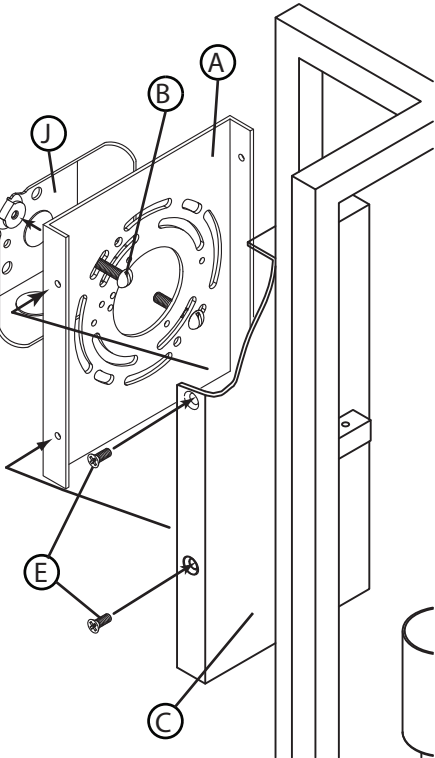
DRAWING 1 - Fixture Installation
