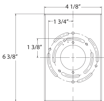
WS-3127/WS-3127F Back Plate Dimensions
