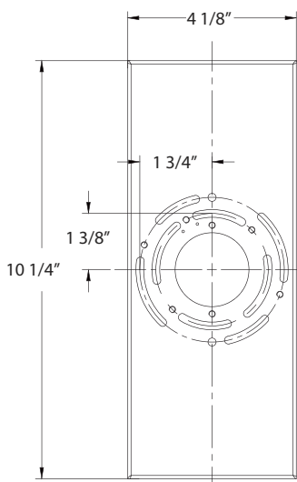
WS-3139/WS-3139F Back Plate Dimensions
