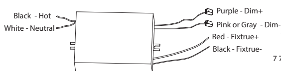
FIG. 3 Driver Wires
