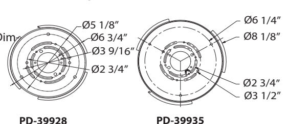
Mounting Plate Dimensions
