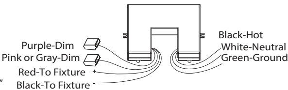
Fig. 3 Driver wires
