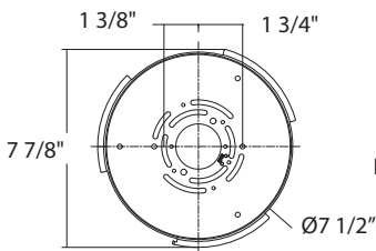
Back Plate Dimensions
