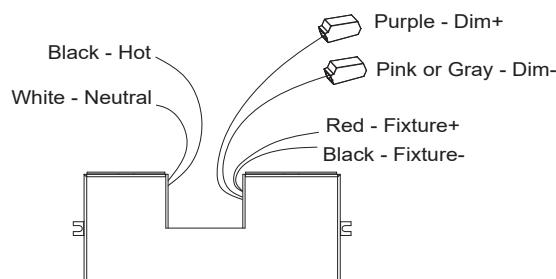
Fig. 3 Driver Wires
