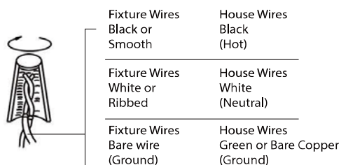
Fig.2 Wiring
