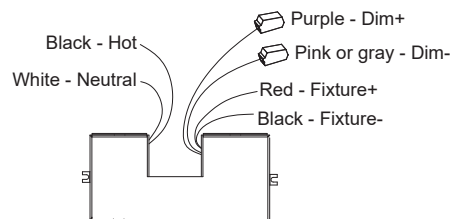
Fig. 3 Driver wires
