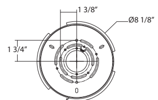
Back Plate Dimensions
