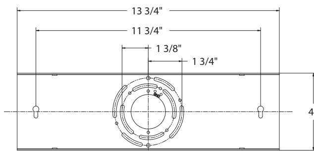
Mounting Plate Dimensions
