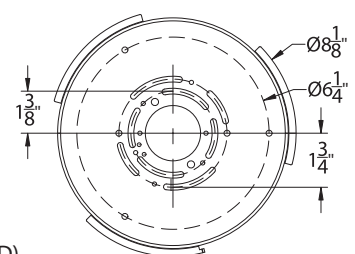
Mounting Back Plate Dimensions
