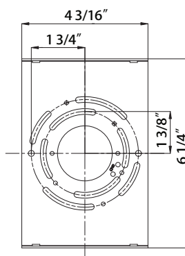
Back Plate Dimensions
