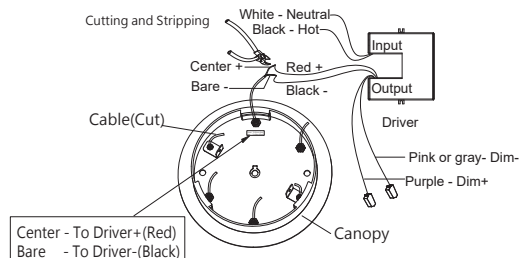
Fig.3 Driver Wires
