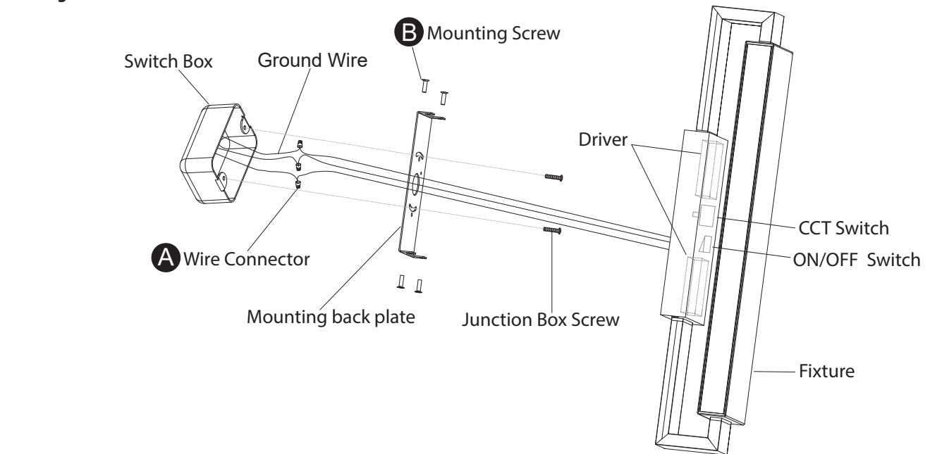
Fig. 1 Mount on Switch Box
